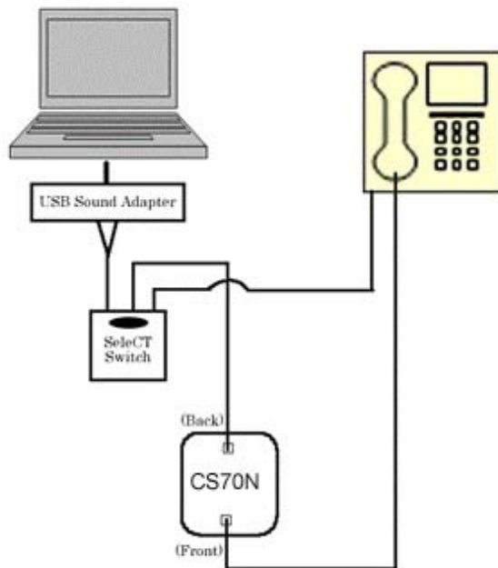
Figure 1: Standard Set-Up
