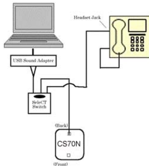
Figure 3: Set-Up with Telephone Having Modular "Headset Jack"
